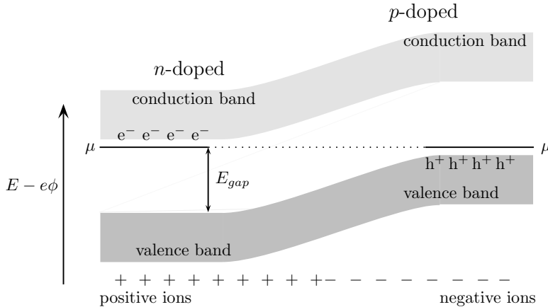
Fig. 18.5 Band diagram of an unbiased p-n junction. This is precisely the same figure as Fig. 18.4, except that the electrostatic potential is added to the band energy. In this figure the equality of the (electro)chemical potential on the left versus the right indicates that there is no net driving force for electrons to flow either left or right. However, in the depletion region there is a net electric field, so if electron-hole pairs are created in this region by absorbing a photon, the electron will flow left and the hole will flow right, creating a net current. Note that the total potential voltage drop over the depletion region amounts to exactly the band gap.
