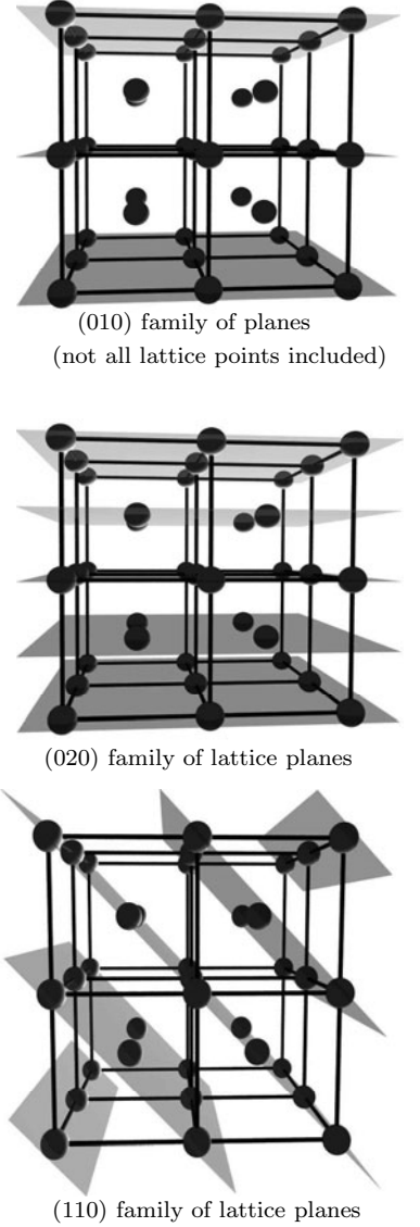
Fig. 13.2 Top: For the bcc lattice, the (010) planes are not a true family of lattice planes since the (010) planes do not intersect the lattice points in the middle of the cubes. Middle: The (020) planes are a family of lattice planes since they intersect all of the lattice points. Bottom The (110) planes are also a family of lattice planes.
