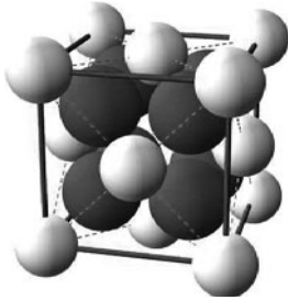
Fig. 14.10 The fluorite structure of \text{PrO}_2 . This is fcc with a basis given by a white atom (Pr) at [0, 0, 0] and dark atoms (O) at [\frac{1}{4}, \frac{1}{4}, \frac{1}{4}] and [\frac{3}{4}, \frac{3}{4}, \frac{3}{4}] .
