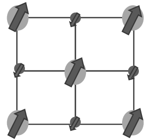
Fig. 20.3 Cartoon of a ferrimagnet. Ordering is antiferromagnetic, but because the different spin species have different moments, there is a net magnetization.
