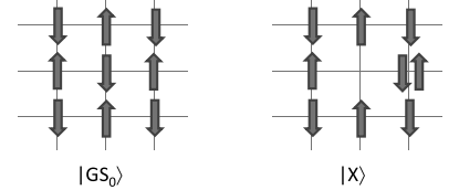
Fig. 23.1 Spin configurations of the half-filled Hubbard model. Left: The proposed antiferromagnetic ground state in the limit that t is very small. Right: A higher-energy state in the limit of small t which can occur by an electron from one site hopping onto a neighboring site. The energy penalty for double occupancy is U .
